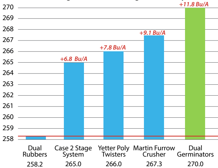
23-24 Averages PTI Farm Closing Wheel Study: No-Till
