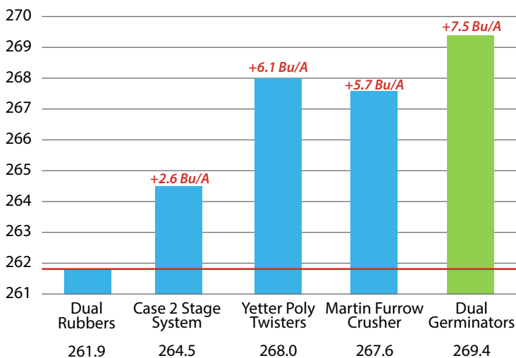
23-24 Averages PTI Farm Closing Wheel Study: Vertical-Till
